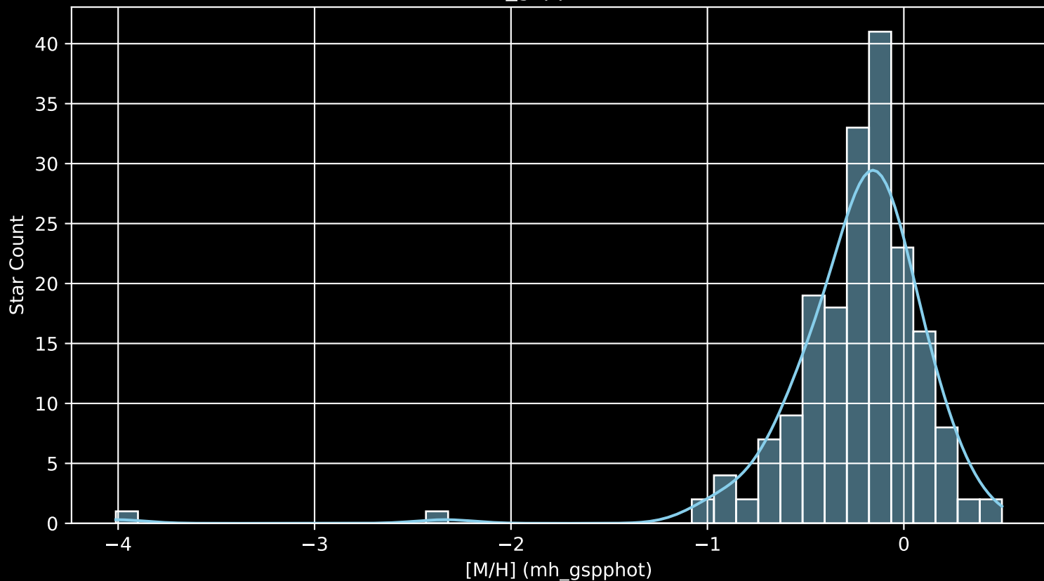
APOGEE DR17 Field: [048-43_MGA [M/H] (mh_gspphot) (n= 188)
