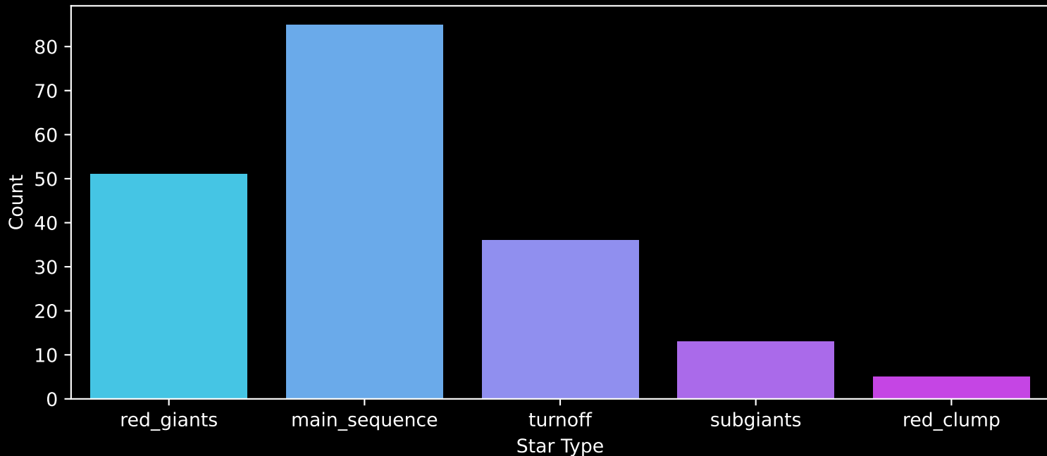
APOGEE DR17 Field: [048-43_MGA] Count plot of Star Type
