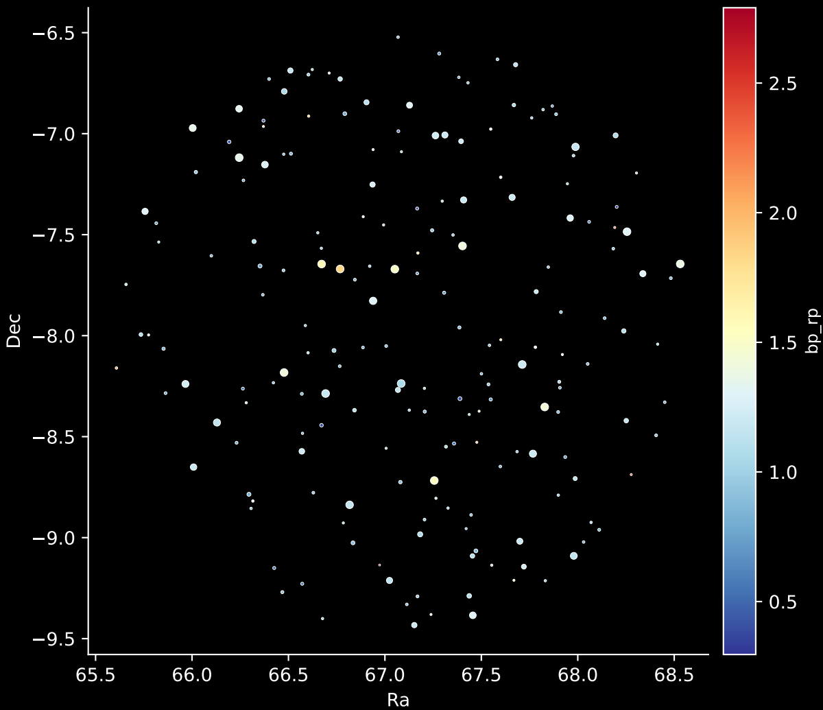
APOGEE DR17 Field: [048-43_MGA] Stars: 190
