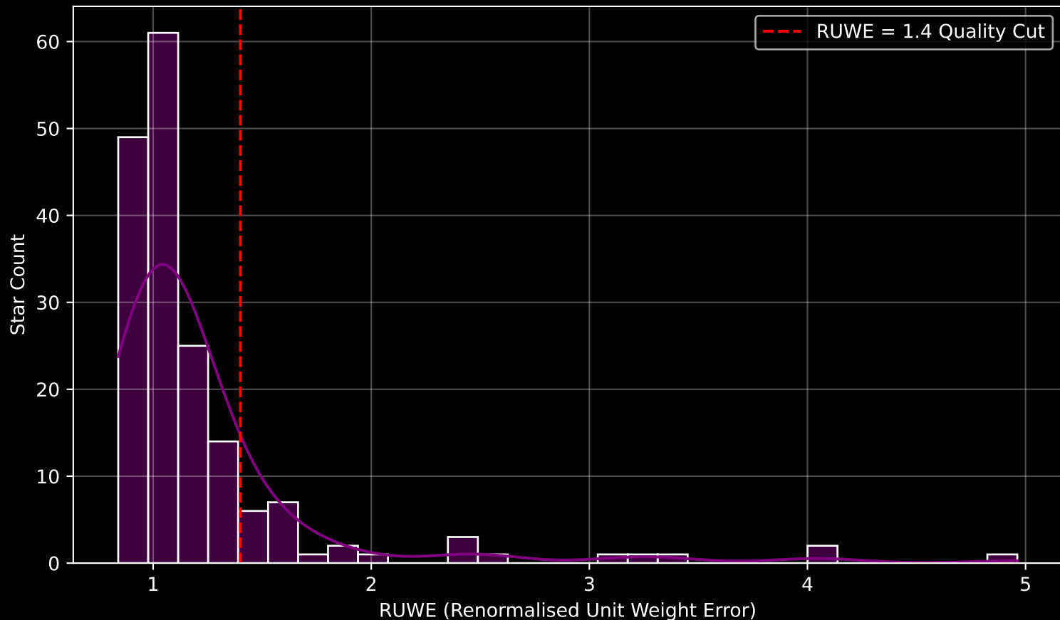
GAPOGEE DR17 Field [048-43_MGA] RUWE Distribution (n= 176)
