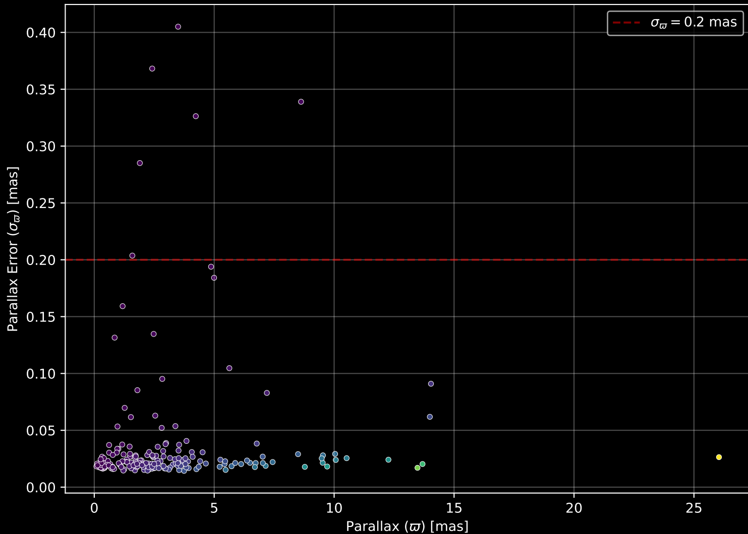
APOGEE DR17 Field: [048-43_MGA] Parallax Quality (n= 190)
