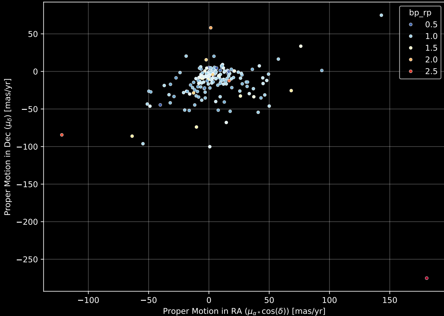
APOGEE DR17 Field: [048-43_MGA] Proper Motion Diagram (n= 190)
